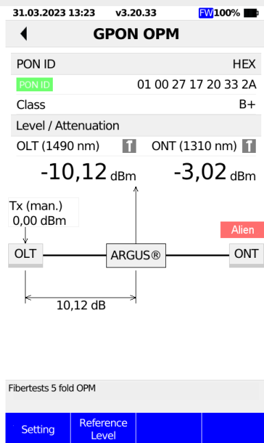
Figure 2: GPON downstream and upstream levels and section attenuation including alien detection, as represented using the ARGUS® F240.
